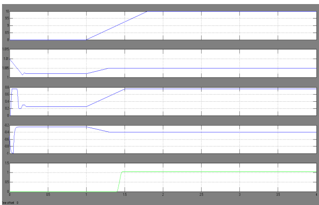
Fig. 10 Simulation results for SCIG system: (a) Wind speed v ; (b) Generator speed \omega_r ; (c) active power P ; (d) reactive power Q ; (e) Pitch angle \beta .
