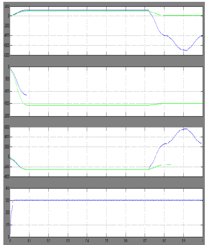
Fig. 8 wave forms of grid, load active and reactive power, inverter Injecting and dc link voltage.
