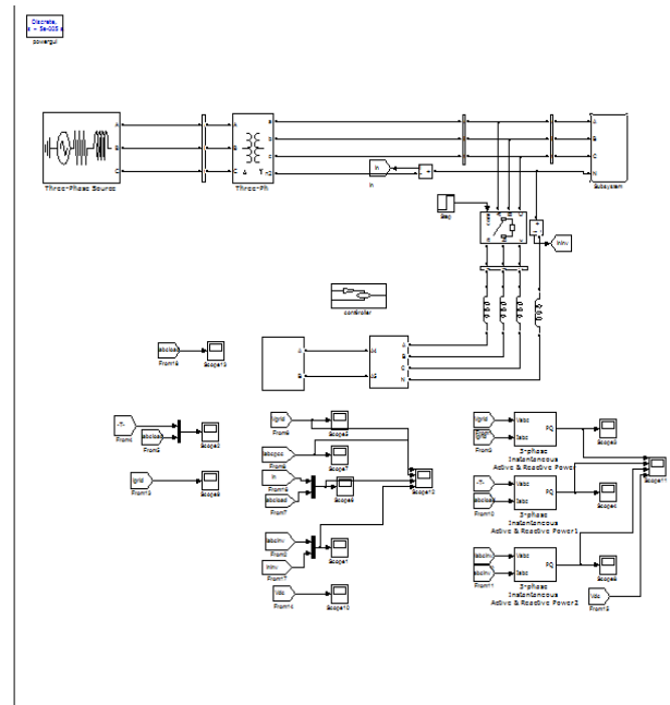
Fig.4 Matlab/Simulink Circuit
