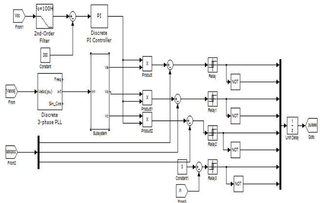
Fig. 5 controller circuit
