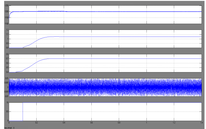
Fig.11 Wind step response. (a) DC-link voltage V_{dc} . (b) Rotor speed \omega_r . (c) Active power P . (d) Reactive power Q . (e) Wind speed v_w .
